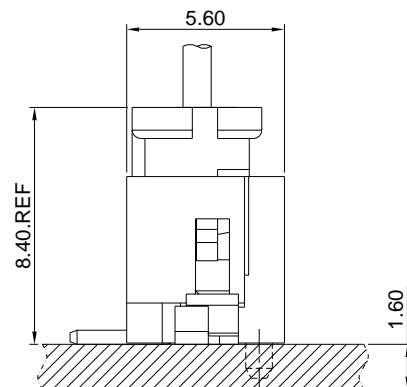
DIP TYPE
