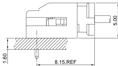
DIP TYPE
